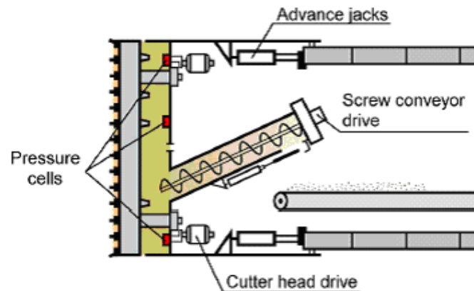
Figure 8: Measurement devices for face support pressure
