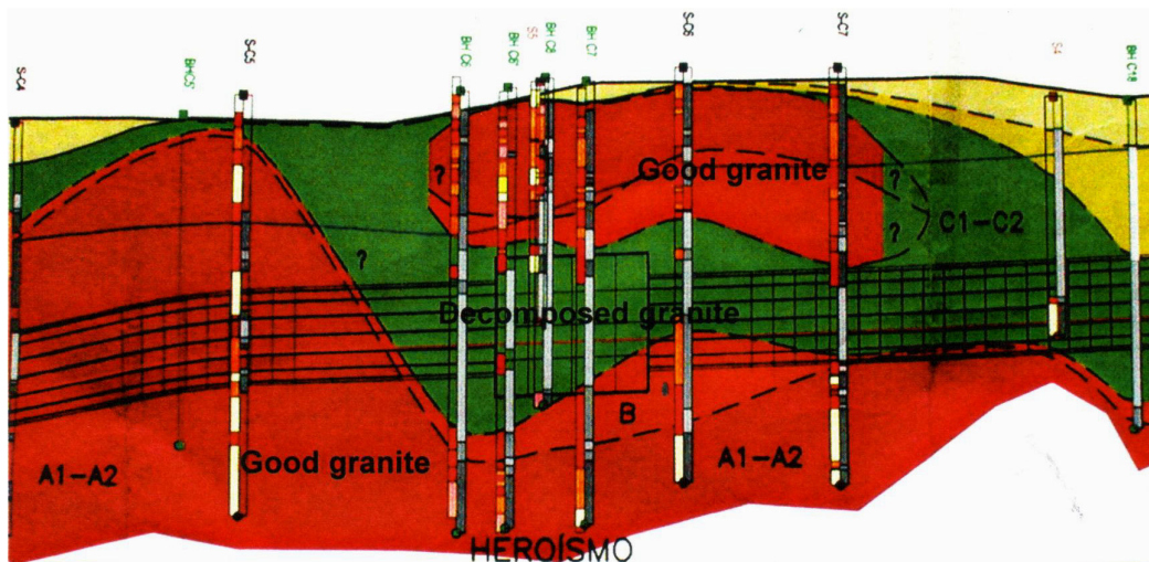
Figure 5: Predicted geology for the Heroísmo mined station (Assessment by Transmetro, documents of Metro do Porto). Heterogeneity in weathering and its erratic geometry is evident.
