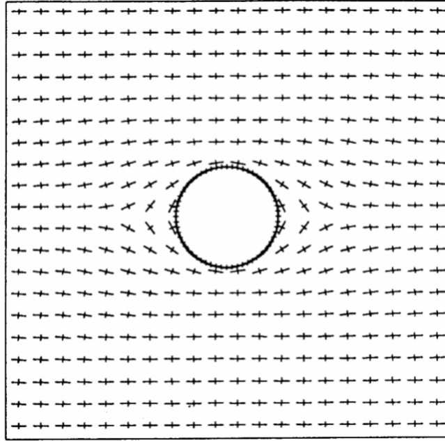
Figure 6: Principal stress directions in the rock surrounding a horizontal tunnel subjected to a horizontal in situ stress \sigma_{h1} equal to 3 \sigma_v , where \sigma_v is the vertical in situ stress.
