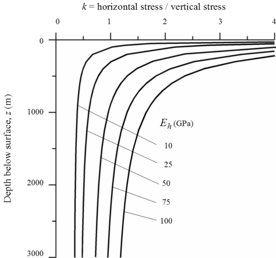
Figure 2: Ratio of horizontal to vertical stress for different deformation moduli based upon Sheorey's equation (Sheorey, 1994).
