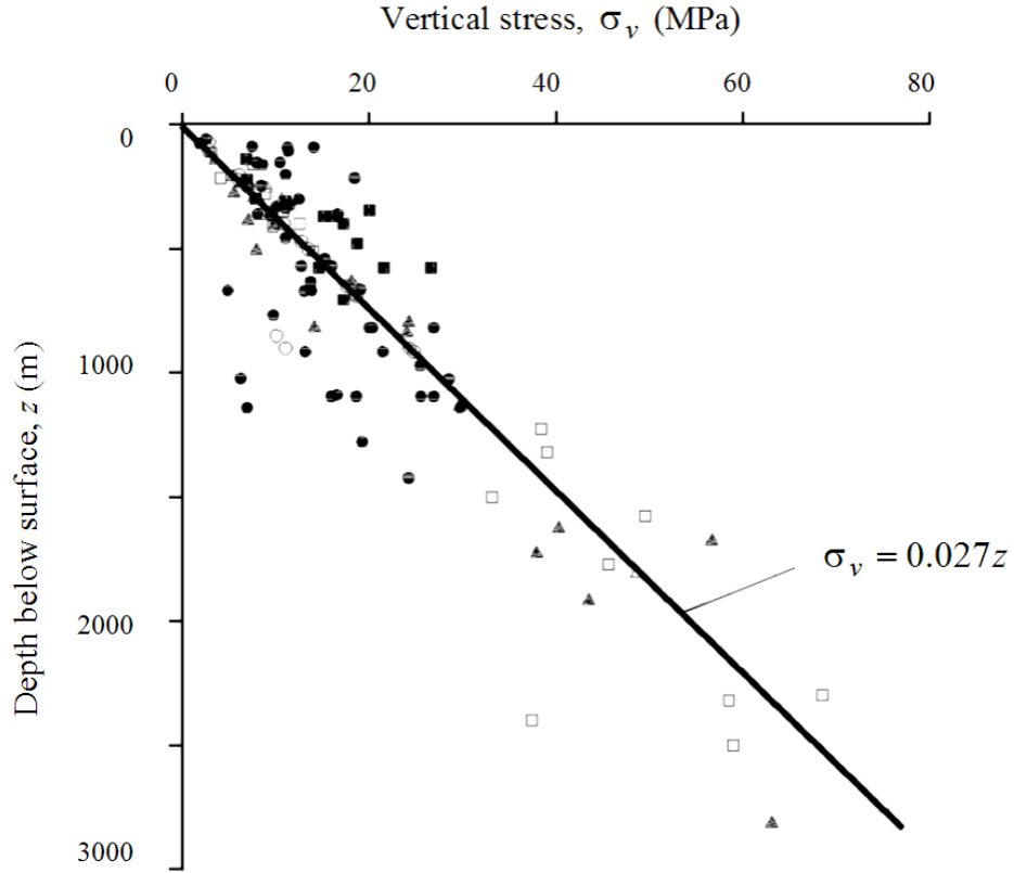
Figure 1: Vertical stress measurements from mining and civil engineering projects around the world (Brown and Hoek 1978).
