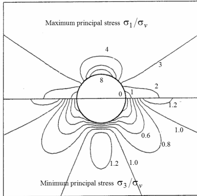
Figure 7: Contours of maximum and minimum principal stress magnitudes in the rock surrounding a horizontal tunnel subjected to a vertical in situ stress of \sigma_v and a horizontal in situ stress of 3 \sigma_v .
