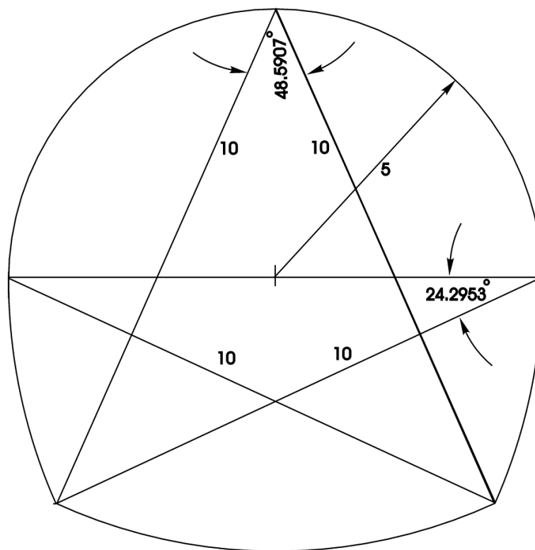
Figure 9: Dimensions of a 10 m span modified horseshoe tunnel shape designed to overcome some of the problems illustrated in Figure 8.
