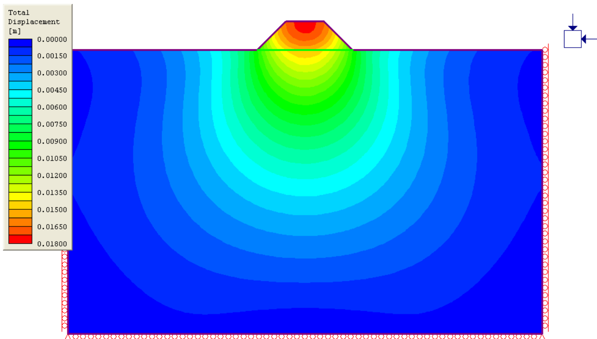
Figure 2: Embankment model – total displacement contours.
