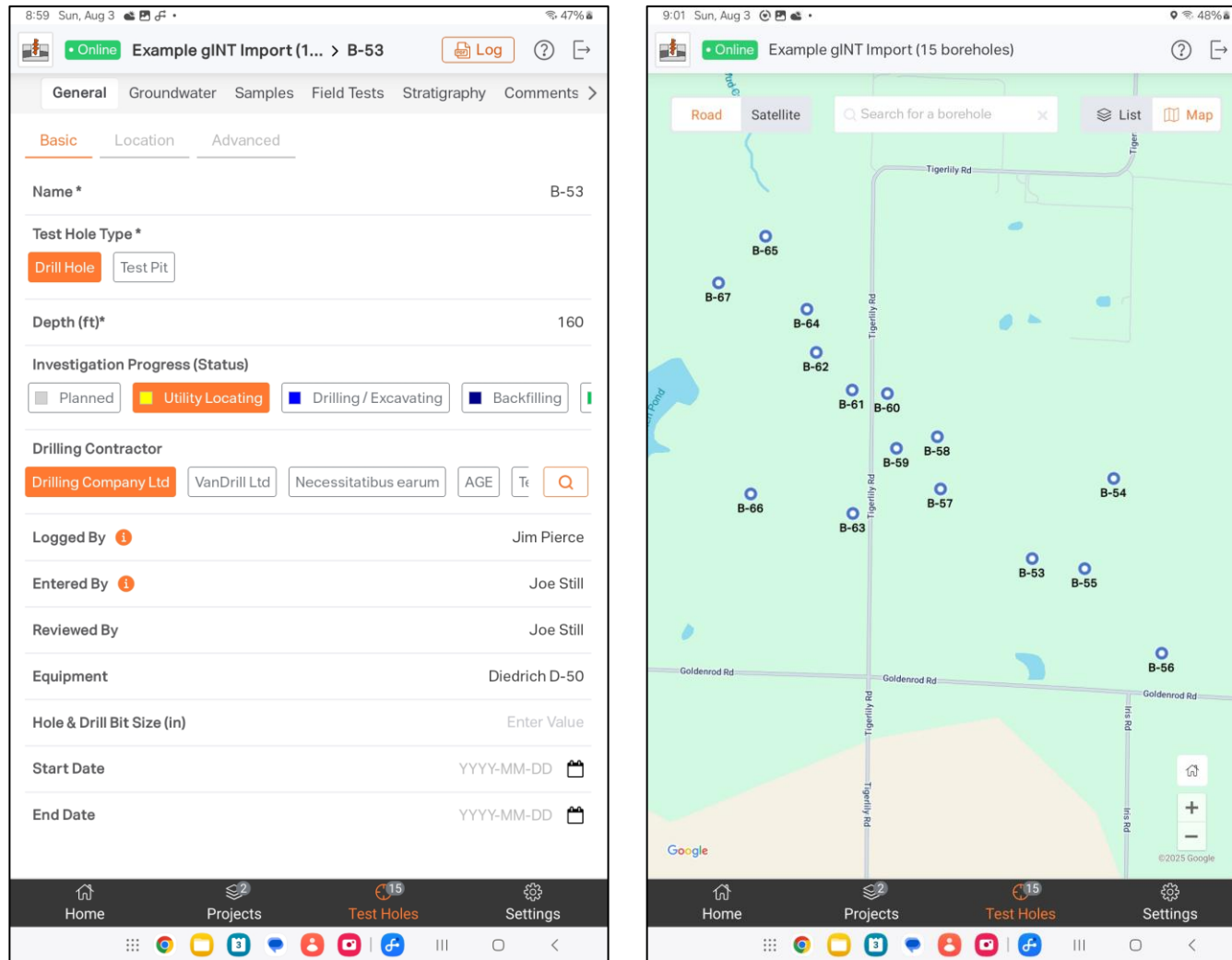
Figure 18: OnSite app (iOS/Android): borehole data entry (left) and map of boreholes (right).
