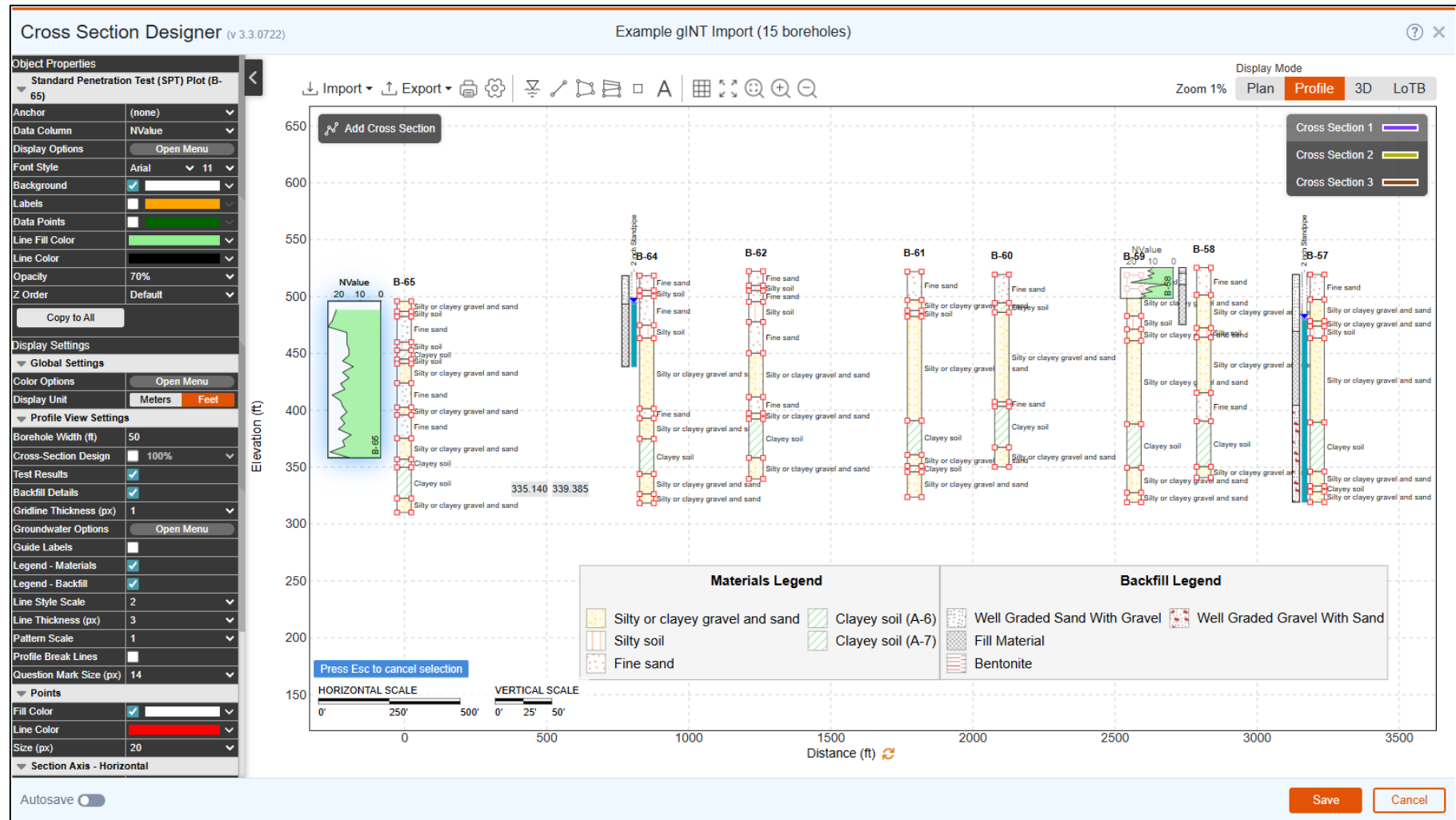
Figure 14: Cross-section designer module in Profile mode (stick logs).
