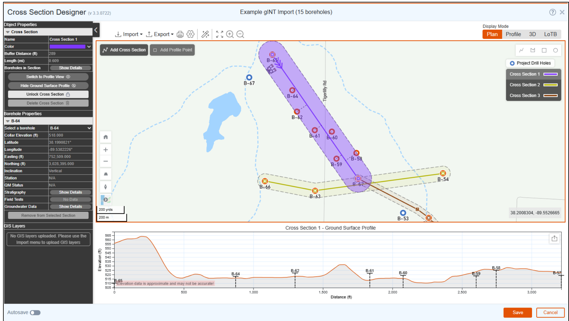
Figure 13: Cross-section designer module in Plan mode.
