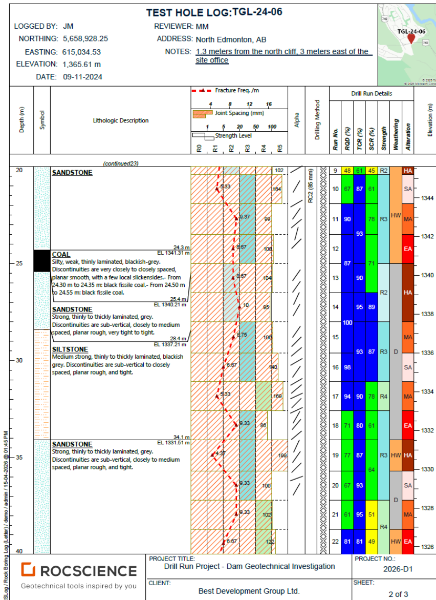
Figure 8: Example of the borehole log generated by RSLog (rock).
