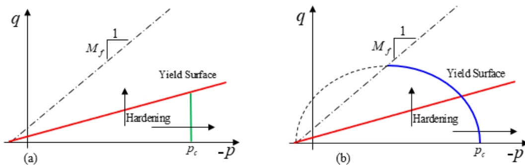
Figure 11.1 - The yield surfaces of the Softening-Hardening model; a) Deviatoric yield surface (red) and the vertical cap (green); b) Deviatoric yield surface (red) and elliptical cap (blue)
