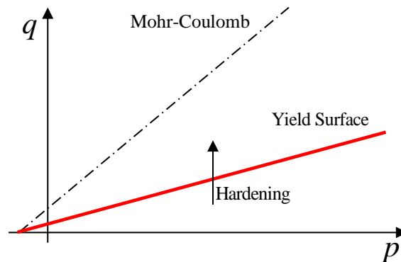
Figure 13.1- The yield surfaces of the CySoil Material Model;
