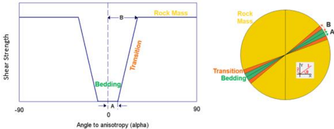
Figure 21.1- Symmetric anisotropy function for Anisotropic Linear model
