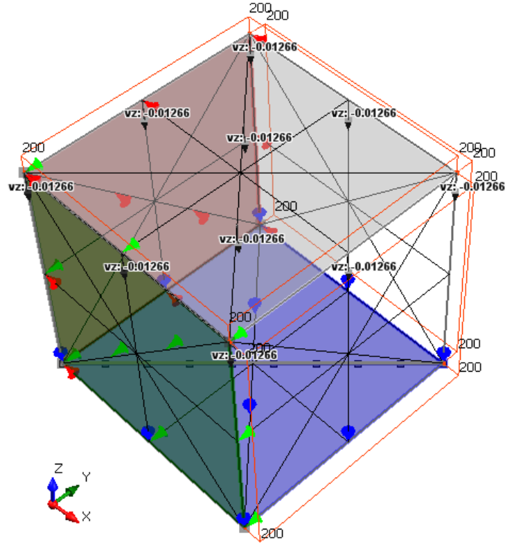
Figure 18-6: Boundary conditions and loads for axisymmetric RS3 analysis; displacement-control control simulation
