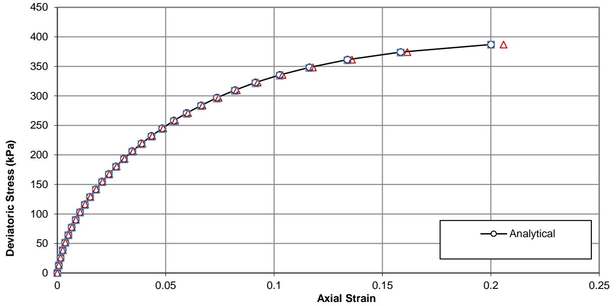
Figure 18-9: Variation of deviatoric stress with axial strain for Example 1 case of constant Poisson's ratio
