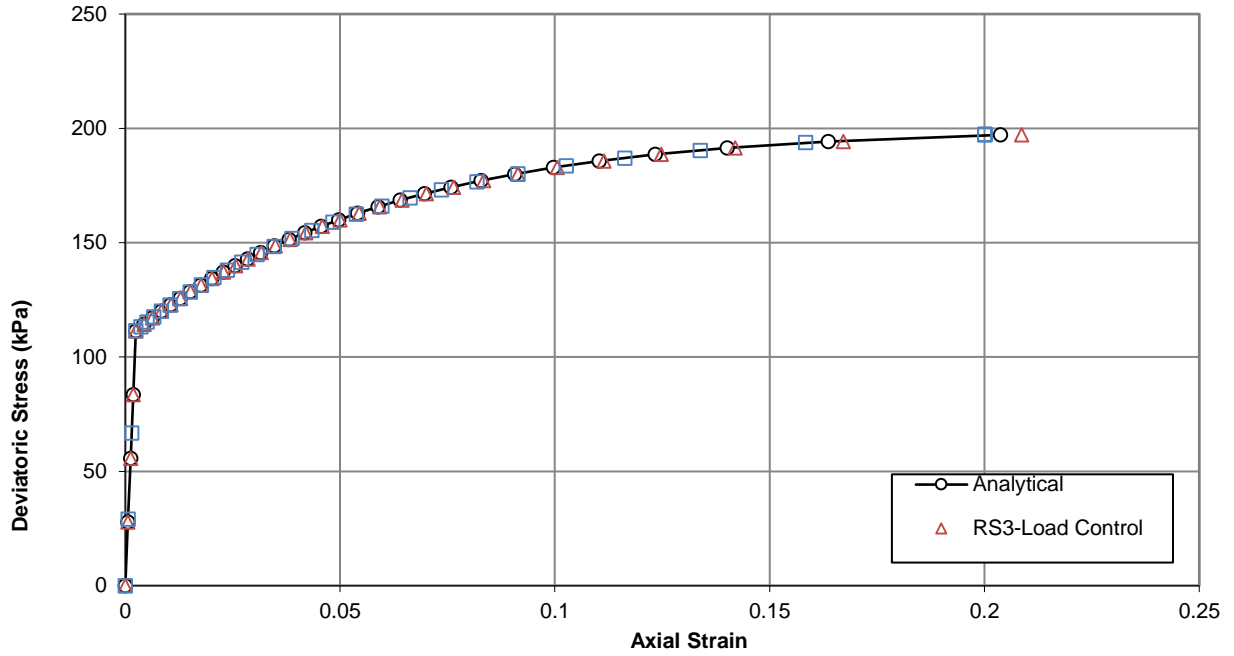
Figure 18-11: Variation of deviatoric stress with axial strain for Example 2 case of constant shear modulus
