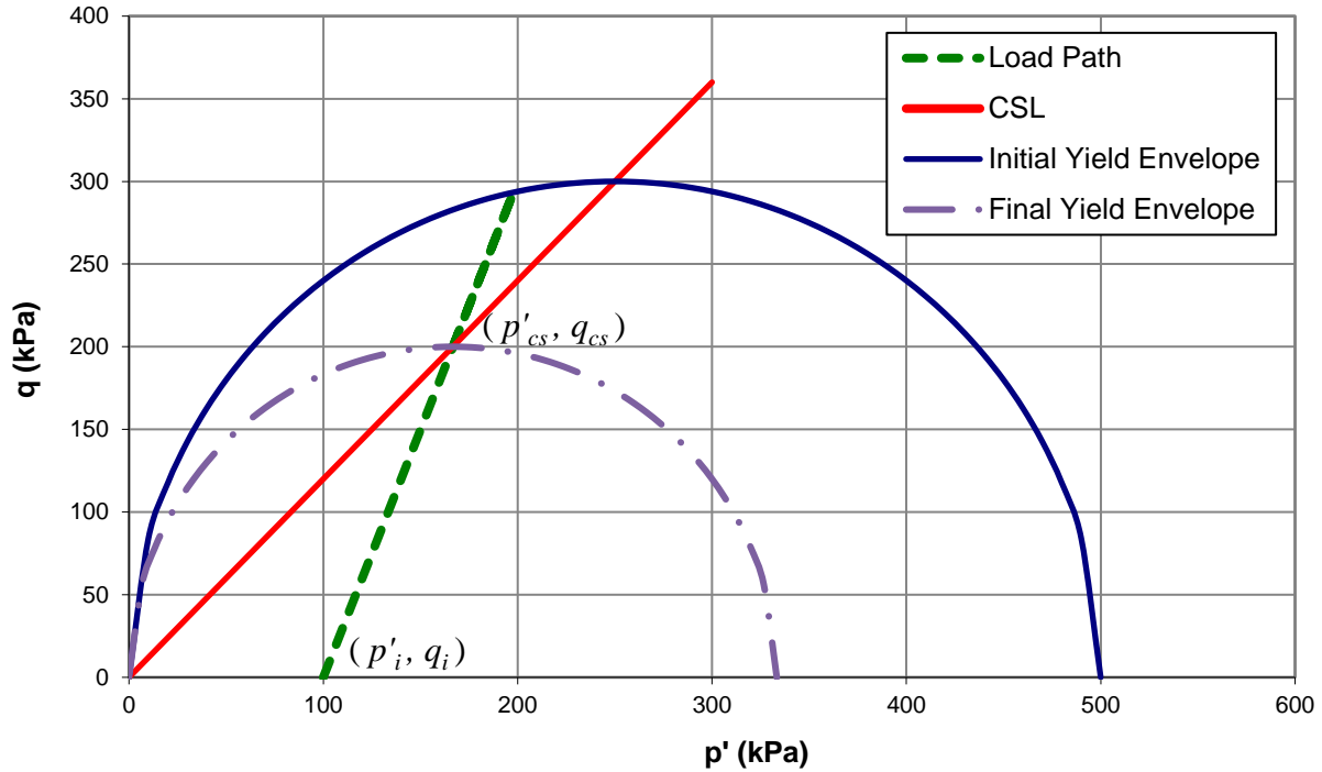
Figure 18-4: Example 3, drained triaxial compressive test on a highly over consolidated clay sample (OCR=5), stress path, initial and final yield surfaces in p'=q' space
