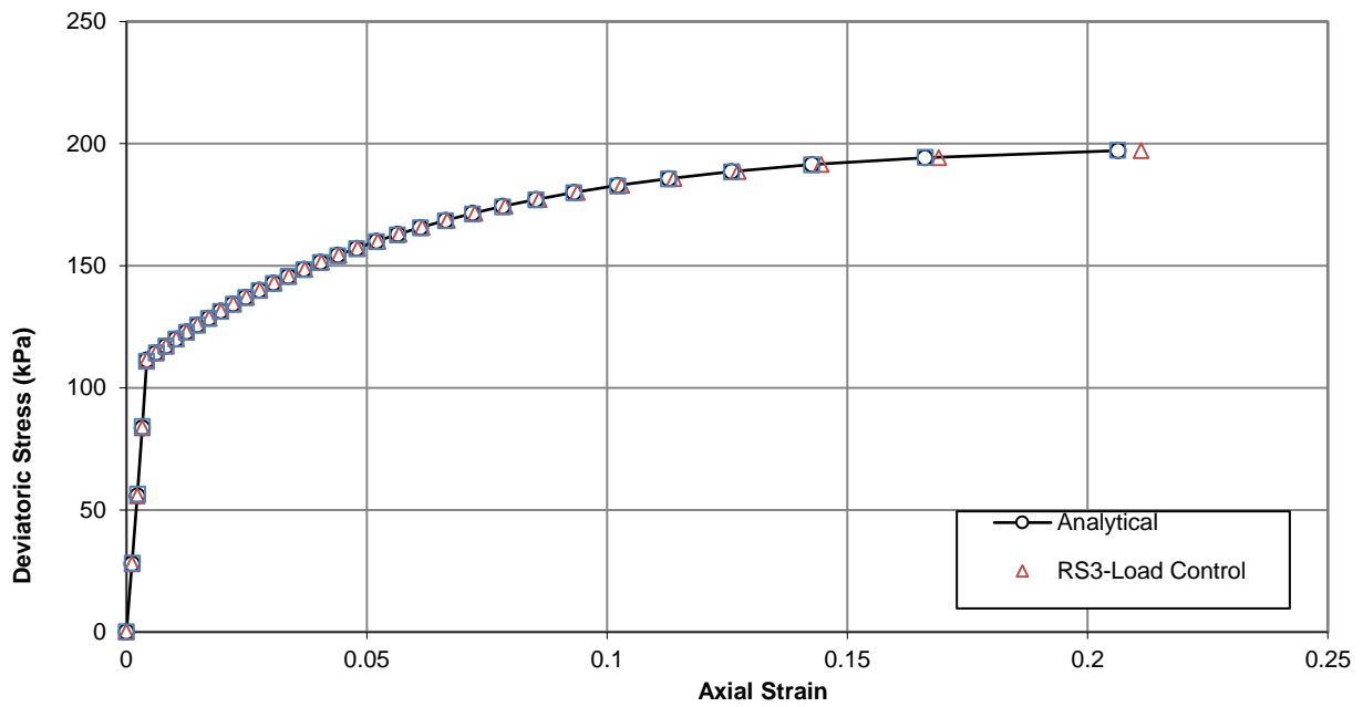
Figure 18-13: Variation of deviatoric stress with axial strain for Example 2 case of constant Poisson's ratio
