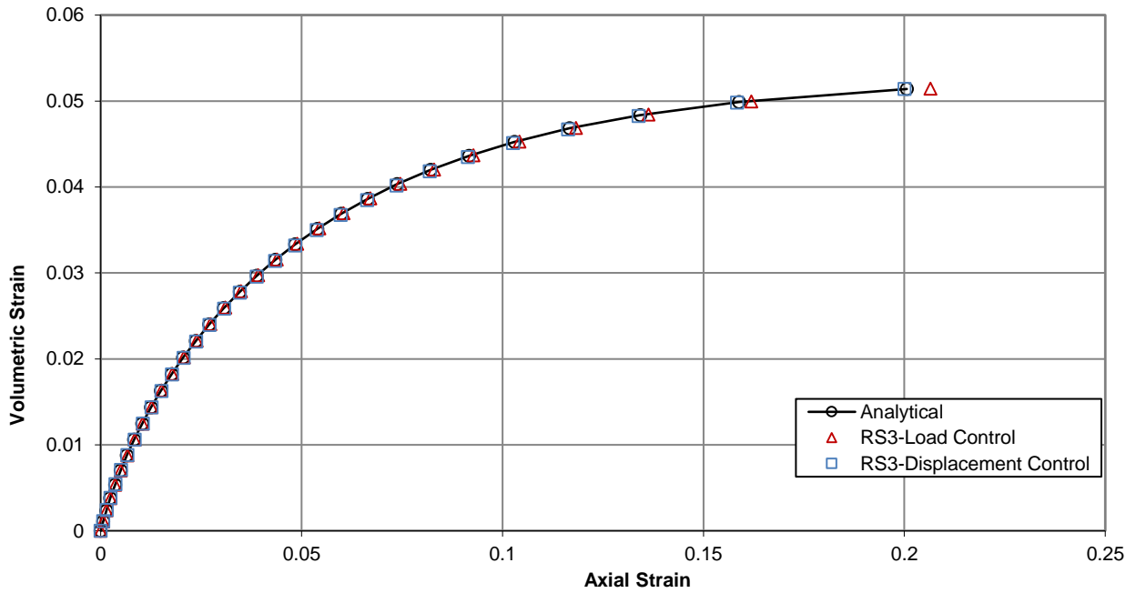
Figure 18-8: Variation of volumetric strain with axial strain for Example 1 case of constant shear modulus
