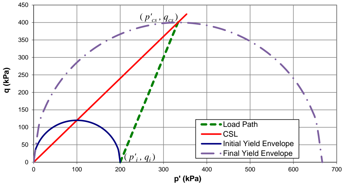
Figure 18-2 : Example 1, drained triaxial compressive test on a normally consolidated clay sample, stress path, initial and final yield surfaces in p' - q space
