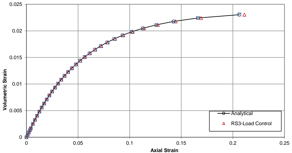
Figure 18-14: Variation of volumetric strain with axial strain for Example 2 case of constant Poisson's ratio
