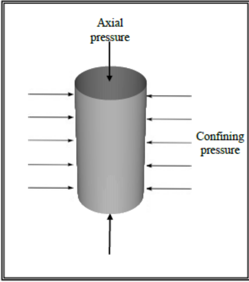
Figure 18-1: Triaxial compressive test of cylindrical soil sample
