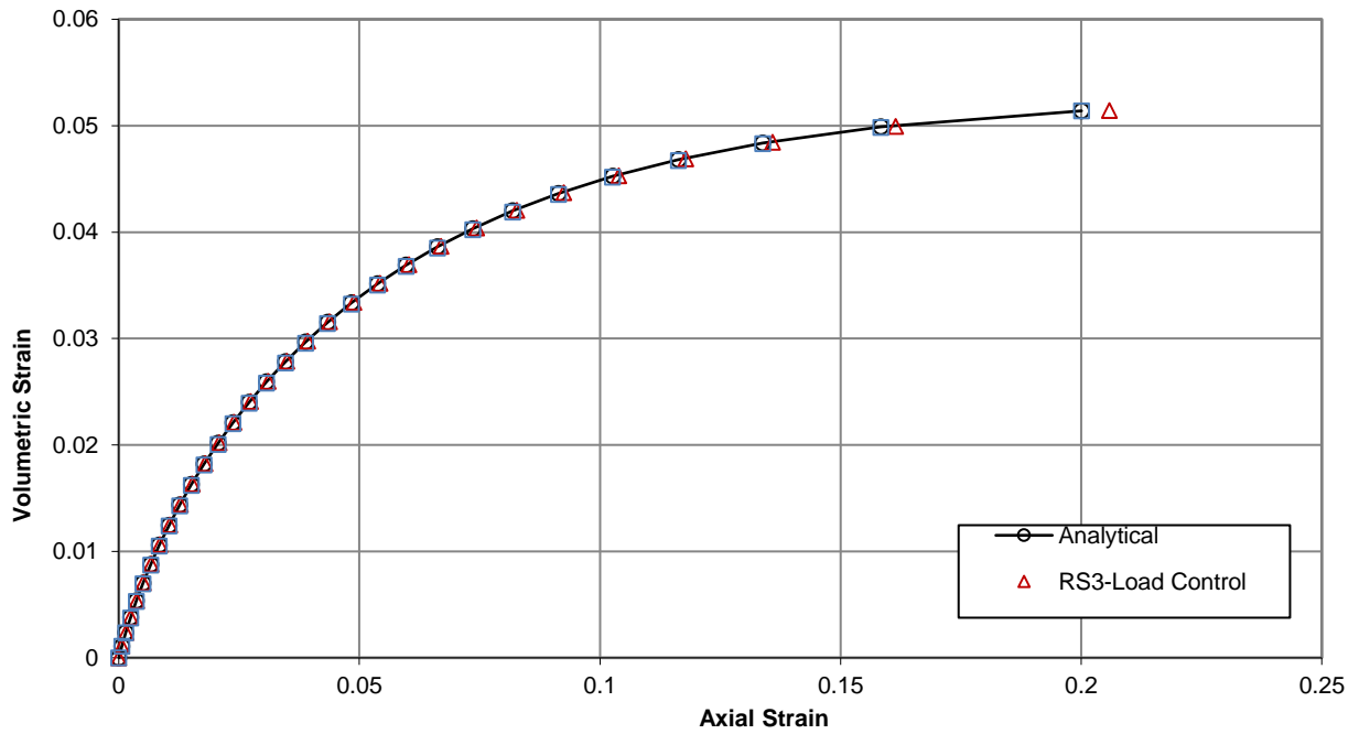
Figure 18-10: Variation of volumetric strain with axial strain for Example 1 case of constant Poisson's ratio
