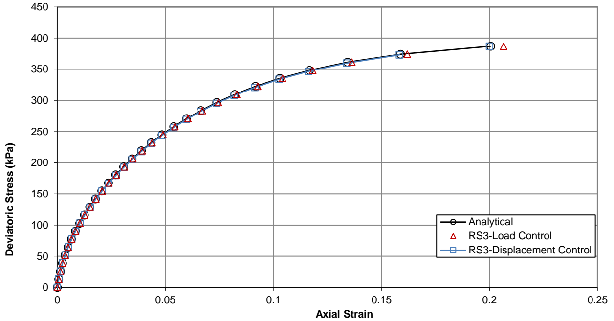
Figure 18-7: Variation of deviatoric stress with axial strain for Example 1 case of constant shear modulus
