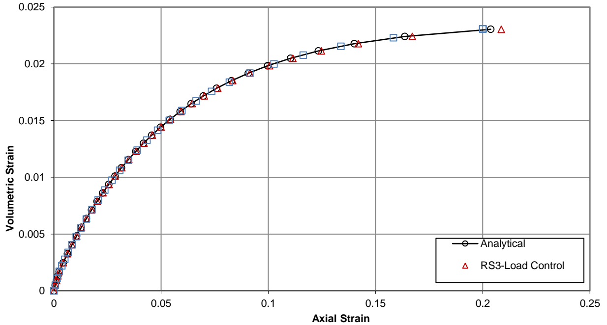
Figure 18-12: Variation of volumetric strain with axial strain for Example 2 case of constant shear modulus
