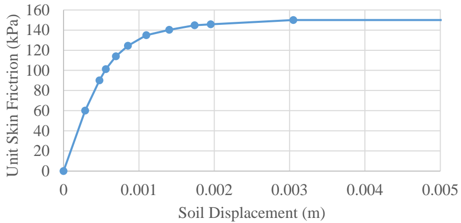
Figure 1-3: Load transfer (t-z) curve for skin friction
