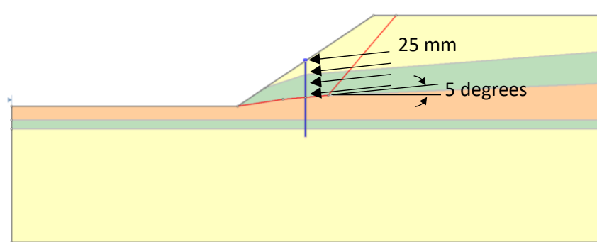
Figure 1-1: Slide model of steel pipe pile subjected to a uniform soil displacement of 25 mm
