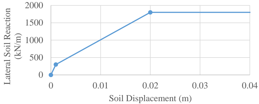
Figure 1-4: Load transfer (p-y) curve for lateral soil reaction
