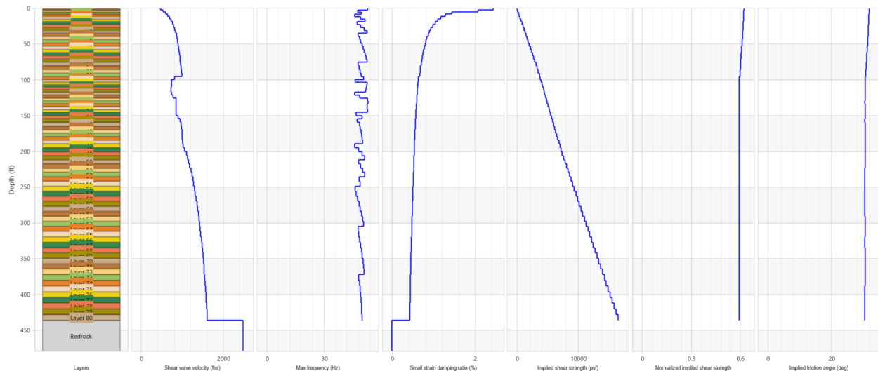
Figure 7.1: Soil Profile with Plots of Key Geotechnical Properties
