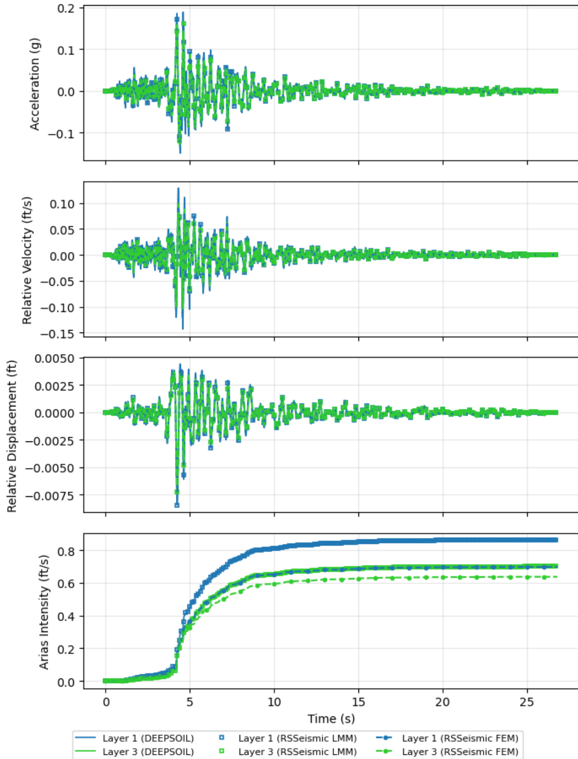
Figure 2.3: Comparison of Time History Plots at Layer 1 and 3 for the Coyote Motion
