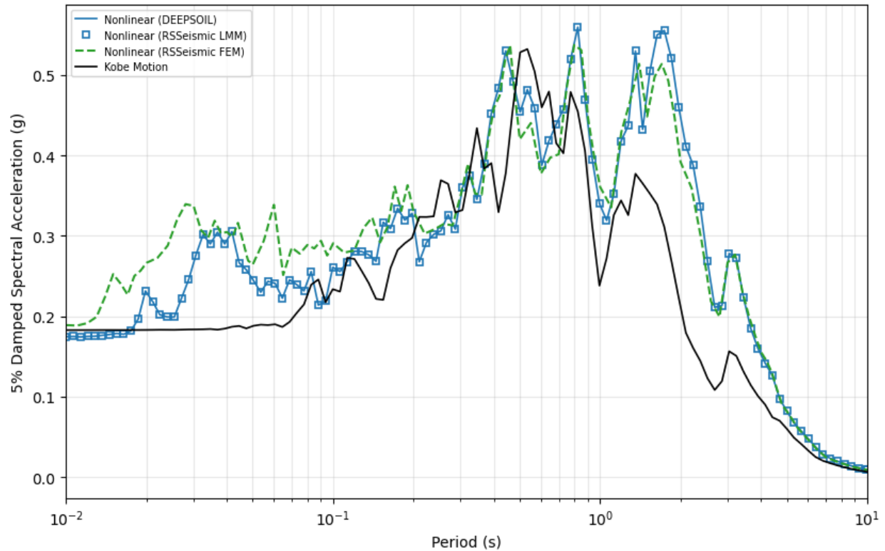
Figure 7.3 below. The lumped mass and finite element analyses show reasonable agreement, with some differences in amplification at lower periods (higher frequencies). The lumped mass RSSeismic and DEEPSOIL analyses show near perfect agreement.
