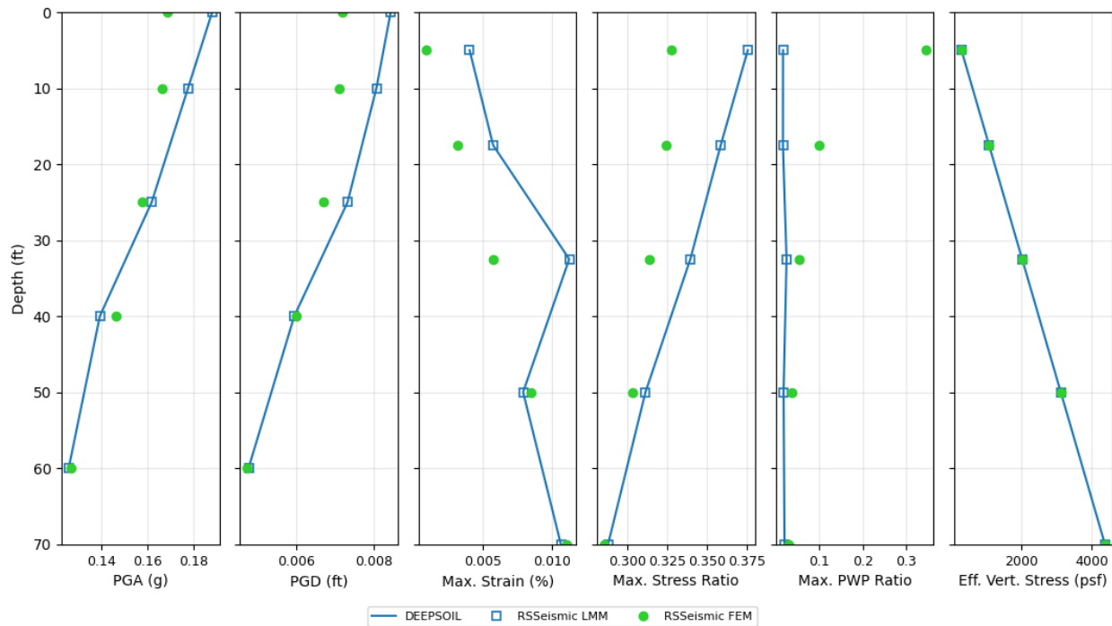
Figure 2.2: Comparison of Profile Plots
