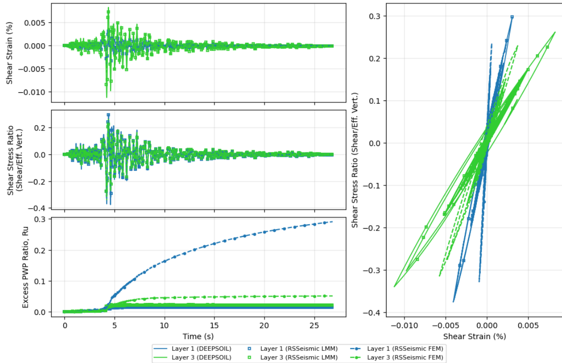
Figure 2.4: Comparison of Stress-Strain Plots at Layer 1 and 3 for the Coyote Motion
