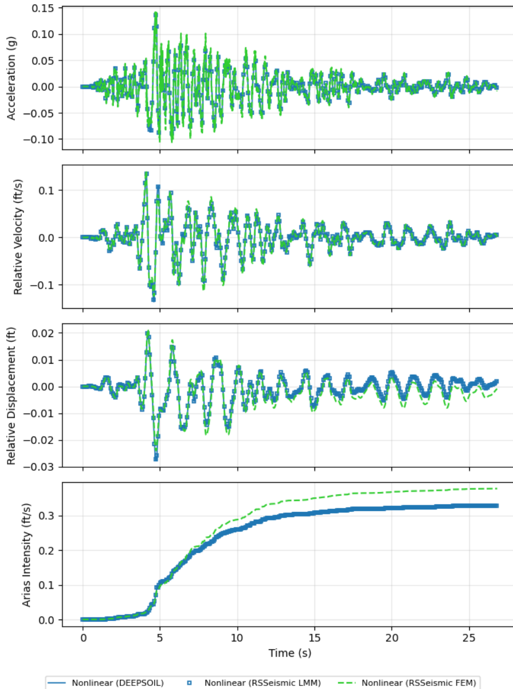
Figure 6.2: Comparison of Time History Plots at the Ground Surface for Nonlinear Finite Element and Lumped Mass Analyses for the Coyote Motion
