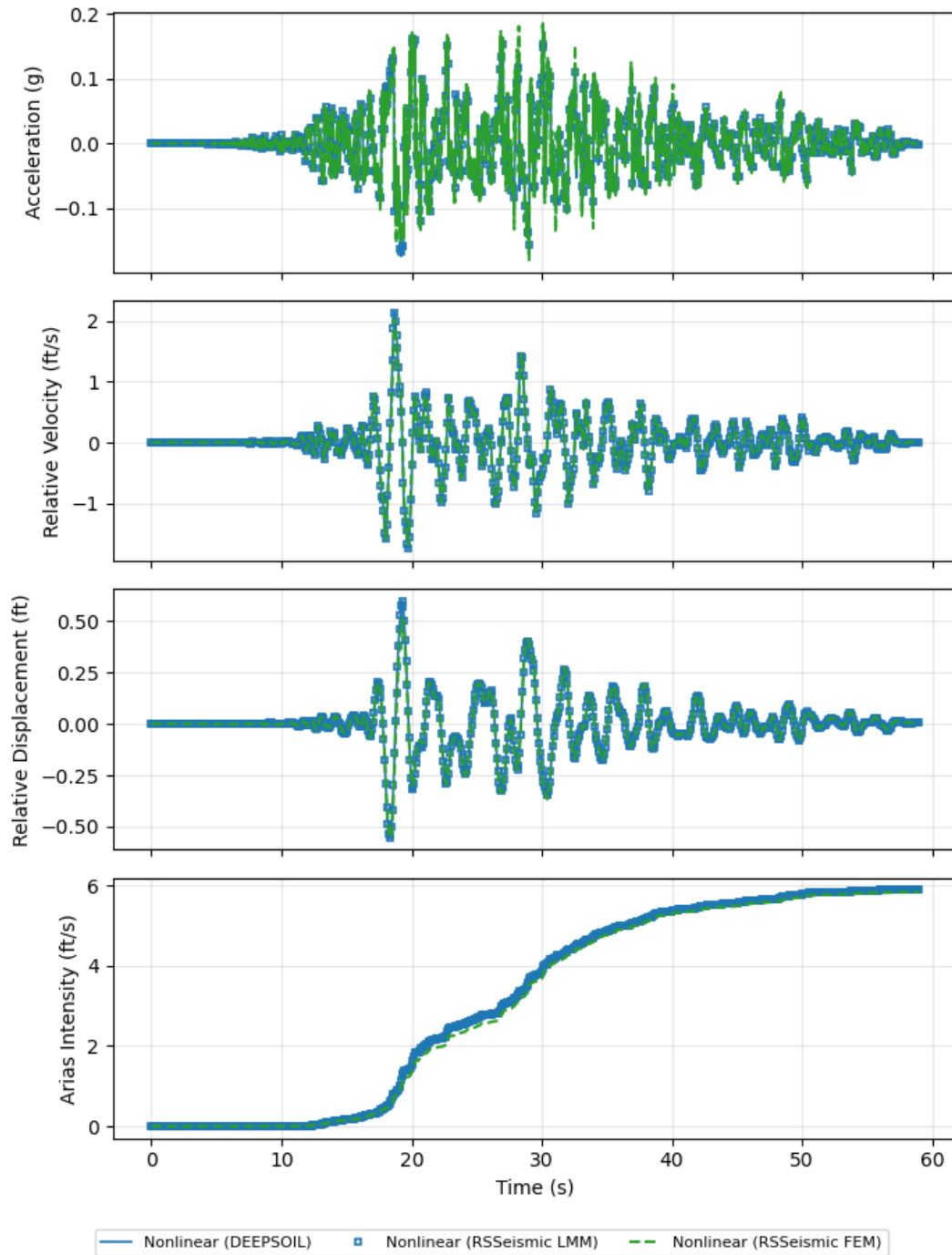
Figure 7.2: Comparison of Time History Plots at the Ground Surface for Nonlinear Finite Element and Lumped Mass Analyses for the ChiChi Motion
