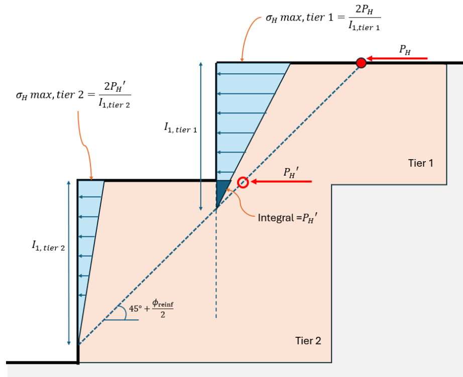
Figure 5.2: Transfer of horizontal loads from upper to lower tier
