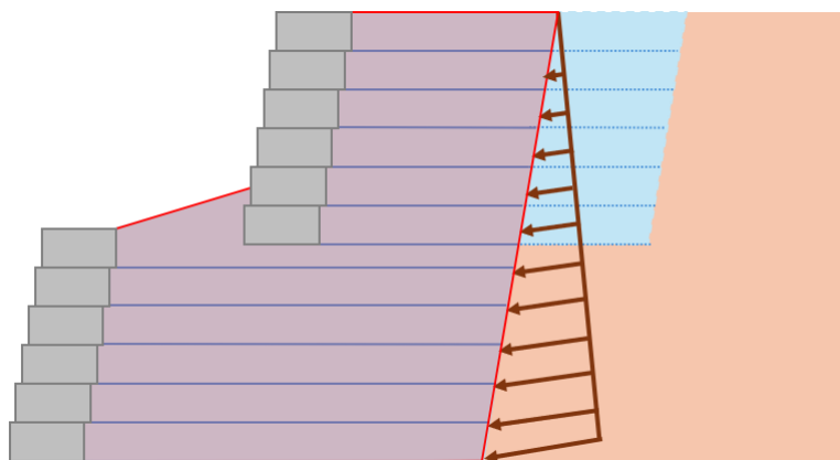
Figure 5.1: Assumed geometry and horizontal earth pressure for external analysis of multi-tier wall
