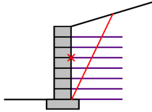
Figure 3.8: Connection strength failure mode
