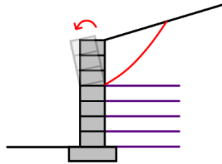
Figure 3.5: Crest toppling failure mode
