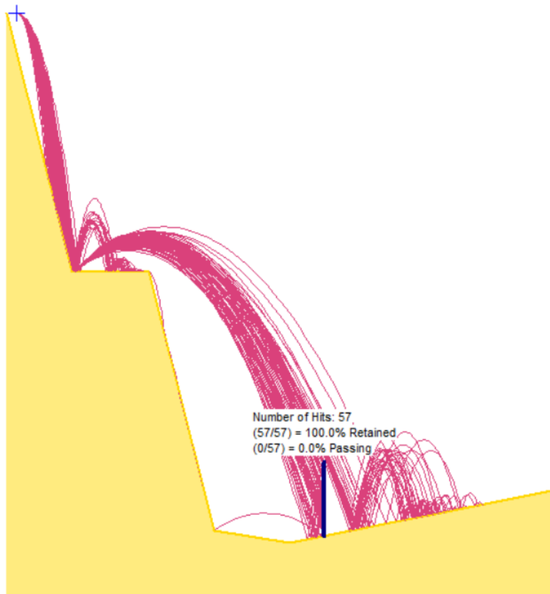
Figure 4-1: RocFall2 Results
